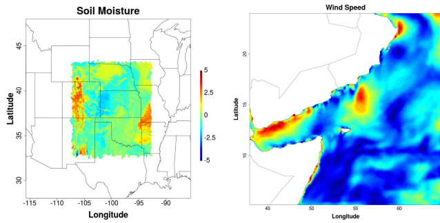
Fig. 4. Left: Soil moisture residuals at the topsoil of the Mississippi River basin. Right: Wind speed (m/s) in the Arabian Sea.
